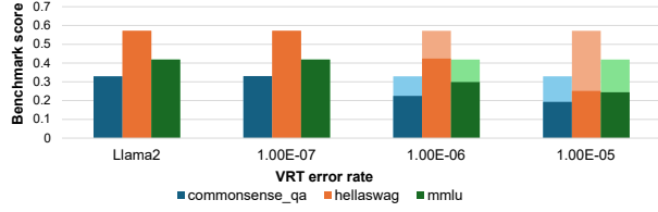
Fig. 14: Benchmark accuracy across varying VRT error rates, with Llama2 baseline. Light and dark bars denote reliable bank-PIM, and dark bars denote bank-PIM with SEC on-die ECC. Random-guess accuracy: commonsense_qa (0.2), hellaswag and mmlu (0.25).
