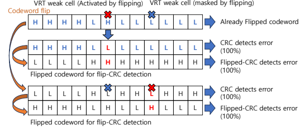
(b) Flip-CRC detection when two VRT weak cells are in different states, demonstrating error detection capability.
