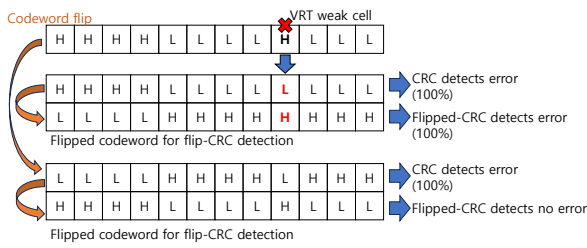
(a) Flip-CRC detection and masking process for one VRT weak cell, showing error detection before and after Codeword Flip.
