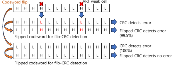
(c) Flip-CRC detection when two VRT weak cells are in the same state, demonstrating error detection capability.
