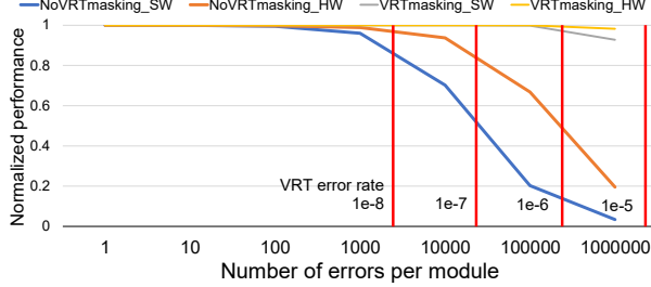
Fig. 13: Reliable-PIM performance across varying VRT error rates; the vertical lines correspond to the VRT error ratios used for the reliability evaluation (Figure 9).
