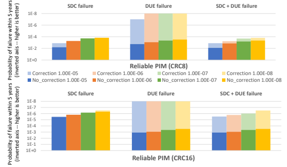
Fig. 11: Reliable bank-PIM SDC, DUE, and SDC + DUE 5-year failure rates; Using the CRC for single-bit correction improves DUE rates substantially.
