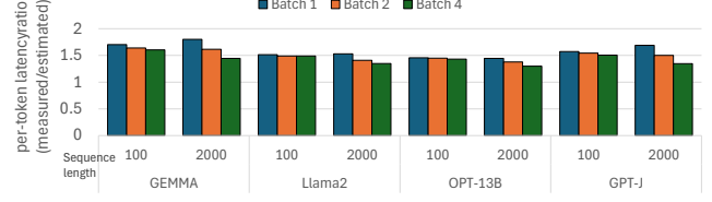
Fig. 8: Measured vs. modeled average per-token decoding latencies for four LLM models on A100 for sequence lengths of 100 and 2000 tokens and a 200-token input.
