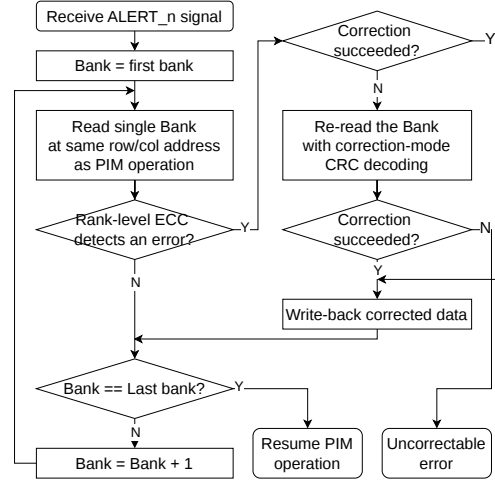
Fig. 4: Host memory controller rank-level correction flow.
