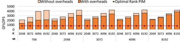
Fig. 12: PIM GEMV microbenchmark performance with various matrix sizes: A is M \times K , B is K \times 1 , and C is M \times 1
