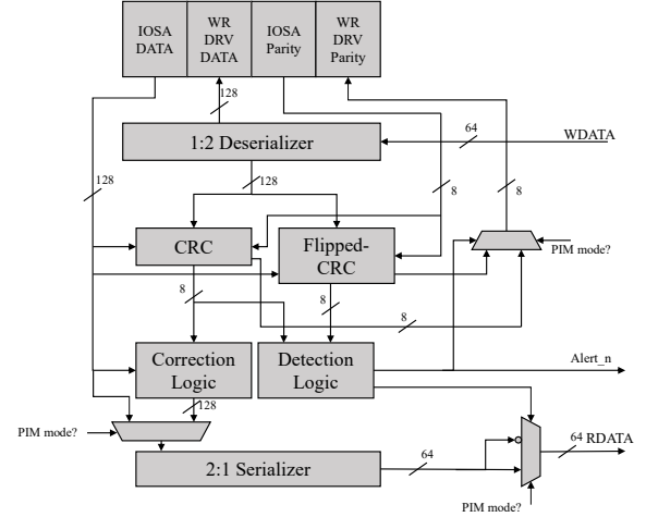
Fig. 5: ECC engine design using the CRC decoder of an adjacent bank as the dual decoder.
