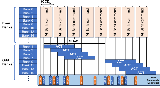
Fig. 7: Odd/even bank pipelining.
