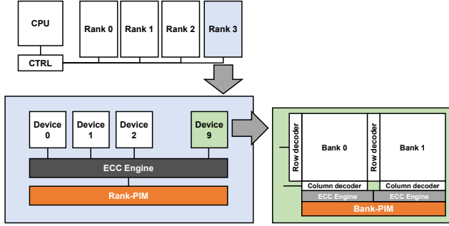
Fig. 2: Rank-PIM and bank-PIM with ECC engines.
