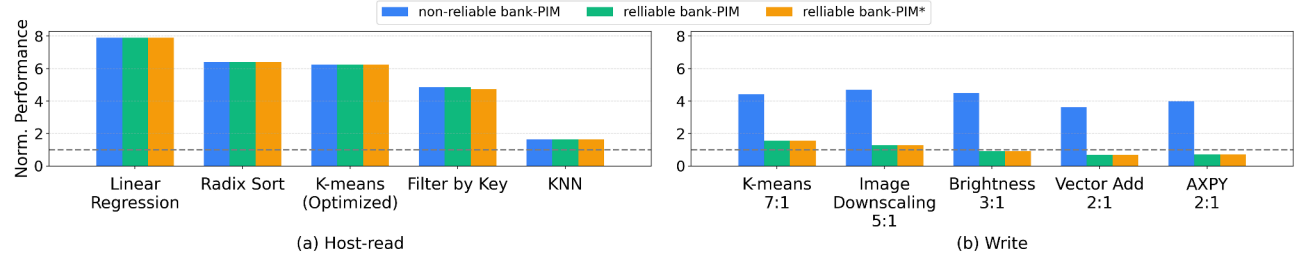
Fig. 16: Performance of bank-PIMs normalized to a rank-PIM under general bank-PIM friendly kernels [1]. (a) Kernels requiring host-side readouts. (b) Write-heavy kernels with read-and-execute to write ratio noted. Reliable bank-PIM refers to error-free performance, while reliable bank-PIM* corresponds to a VRT error rate of 10^{-5} performance.
