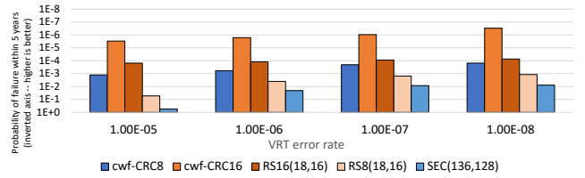
Fig. 10: SDC failure rates with various types of on-die codes: cwf-CRC8 and cwf-CRC16 use our Codeword Flip mechanism with 8-bit or 16-bit CRC dual decoding to both detect and mask VRT errors (after rank-level correction). The other codes attempt error correction in DRAM, but still rely on the second-tier rank ECC for better reliability.
