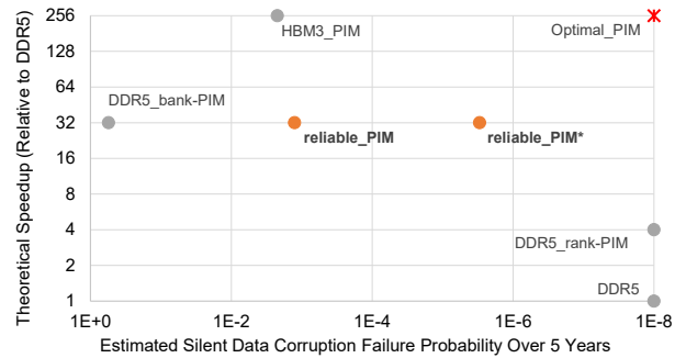
Fig. 1: Modeled reliability vs. theoretical max speedup for standard rank-PIM and bank-PIM in a one channel, 4 rank system; reliable_PIM uses DDR5 on-die ECC redundancy, and reliable_PIM* aligns with HBM3 on-die ECC redundancy.
