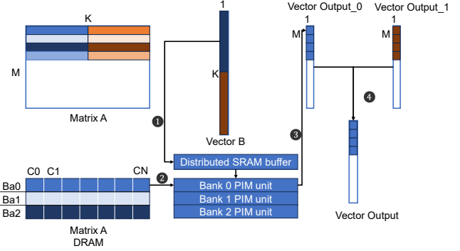
Fig. 3: GEMV operation flow in bank-PIM.
