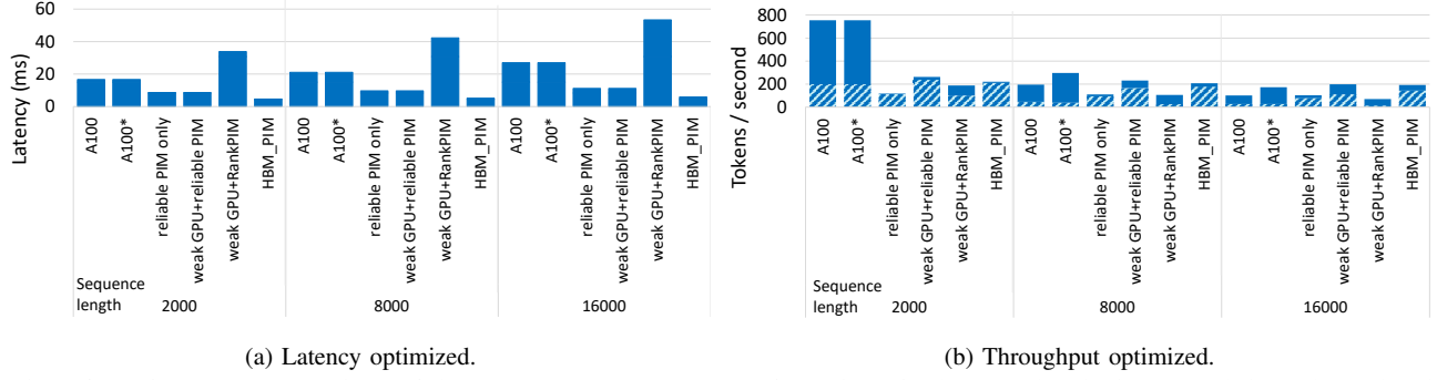
Fig. 15: Performance comparison of the OPT13B LLM across configurations for latency (batch size 1) and throughput (batch size bound by KV cache capacity) optimized execution. The bottom (patterned) portion of each throughput bar shows the fraction of execution time spent on feed-forward GEMM operations while the top (solid) is the GEMV self-attention portion.
