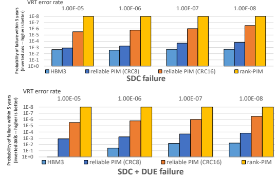
Fig. 9: SDC and SDC+DUE rates over 5 years comparing a reliable bank-PIM, an HBM3 bank-PIM, and a rank-PIM (inverted y-axis—higher bars indicate better reliability).
