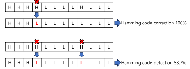
(d) Hamming(136,128) code performance on single and double bit errors, highlighting significant error rate challenges.
